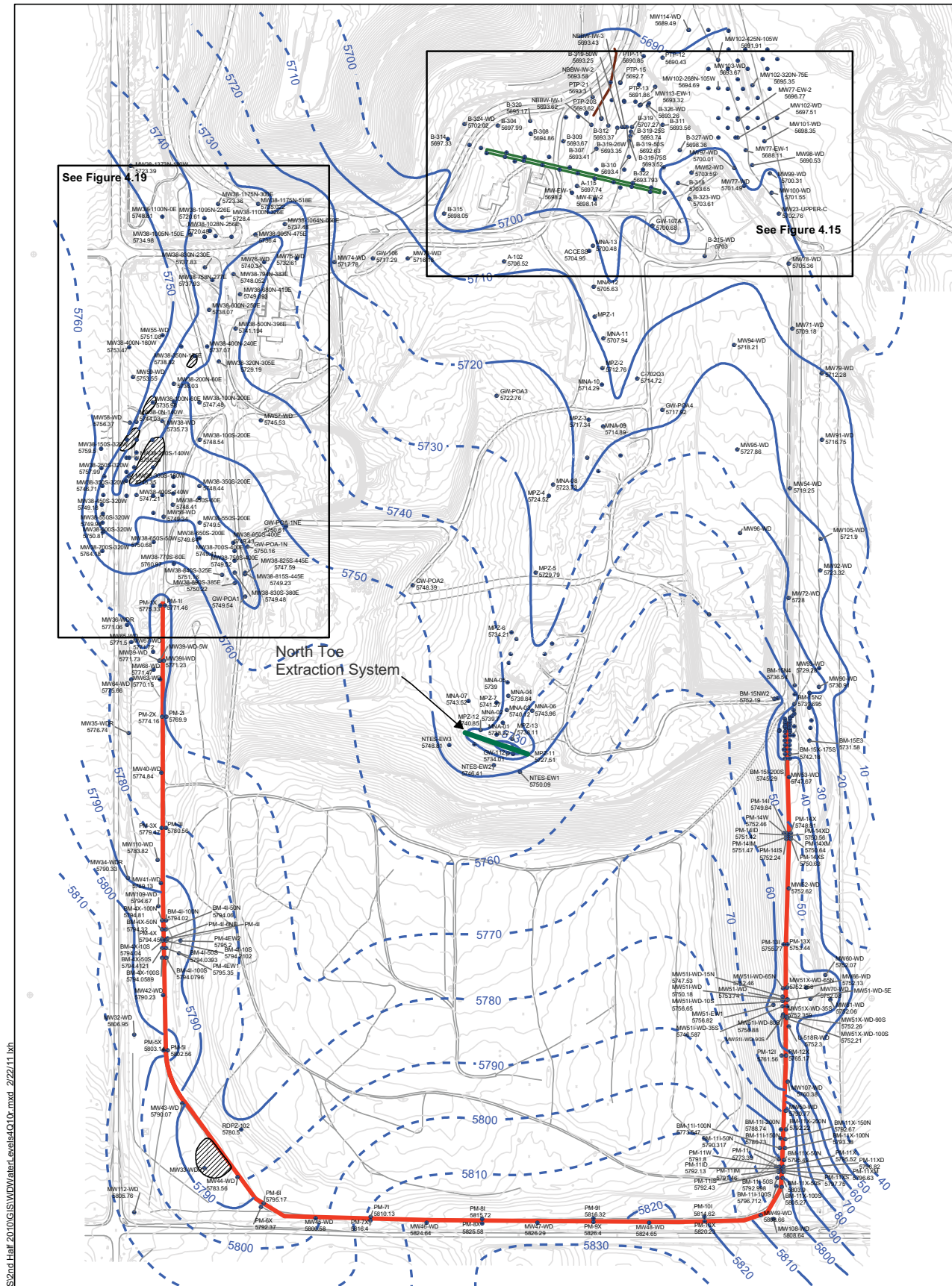
FIGURE 4.2 SITEWIDE POTENTIOMETRIC SURFACE ALLUVIUM/WEATHERED DAWSON October 4 - 12, 2010 O&M Status Report - 2nd Half 2010 Lowry Landfill Superfund Site
